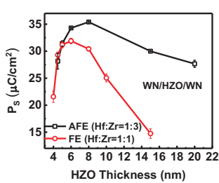
Fig. 9. P_s scaling metrics of AFE and FE HZO with WN electrodes.
